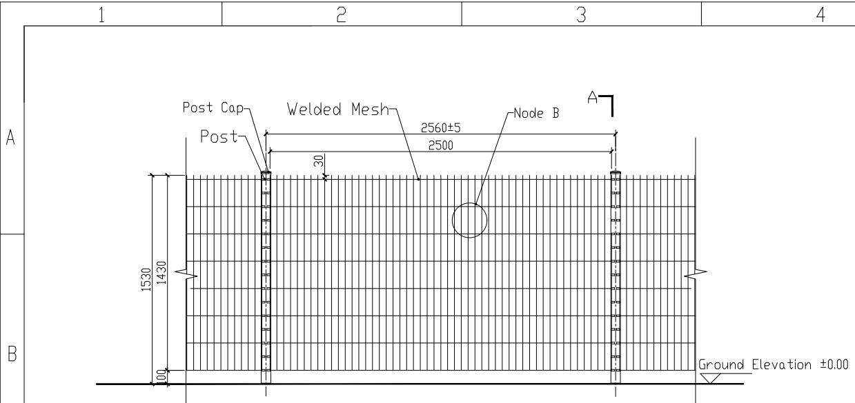
Fence Elevation A-A
