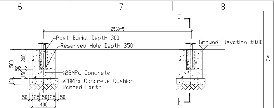
Foundation Elevation
