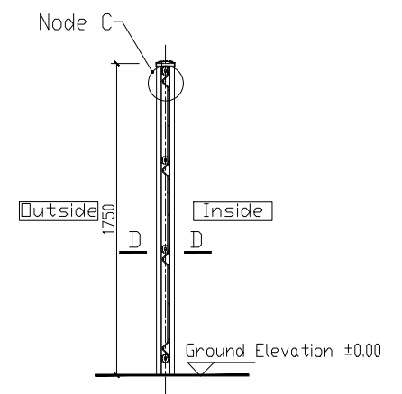
A-A Sectional
