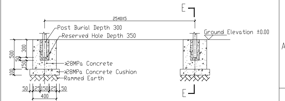
Foundation Elevation
